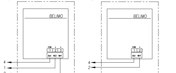
Optional Outdoor Air Damper Actuator: Optional Exhaust Air Damper Actuator:
