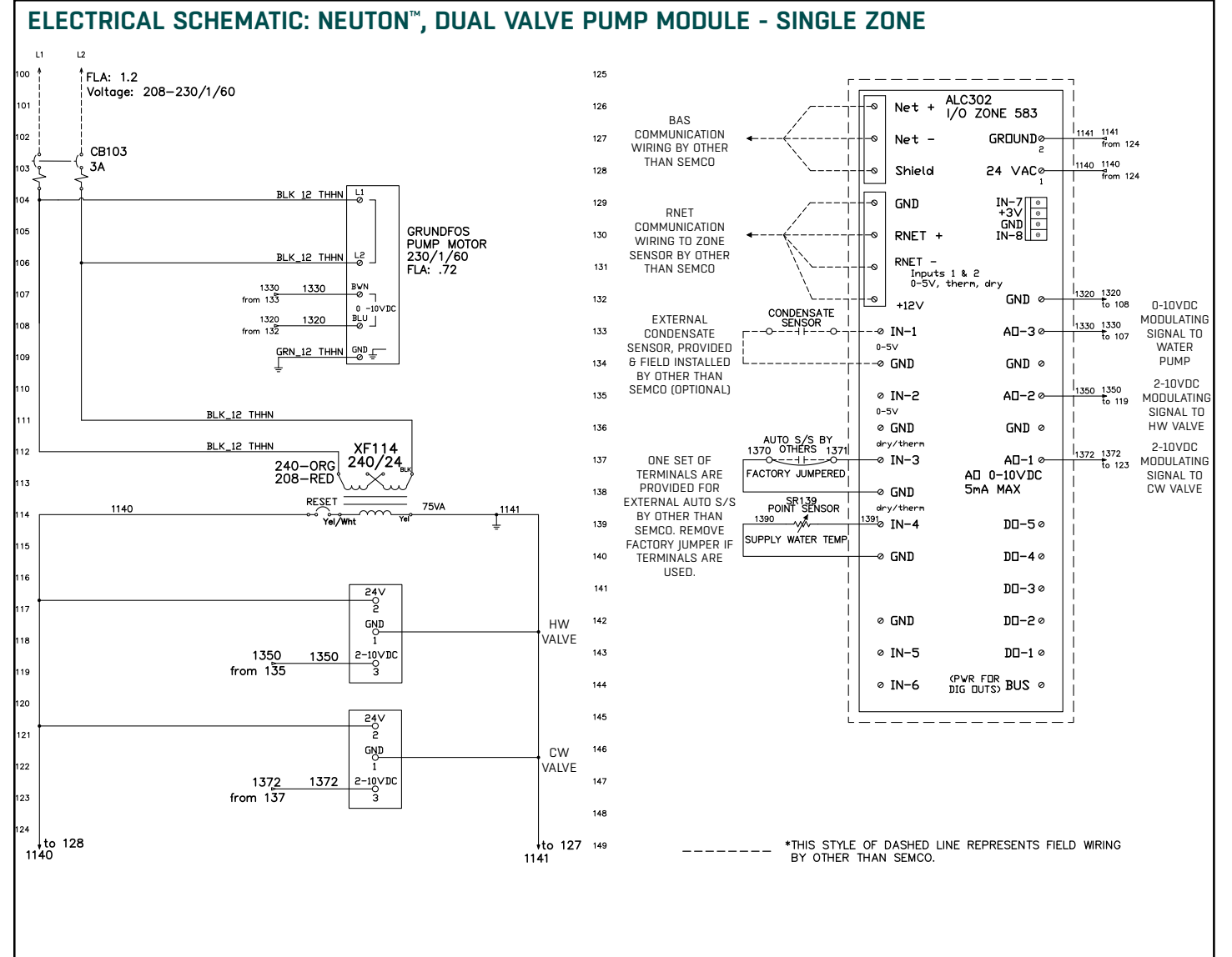
FIGURE 11. Electrical schematic for NEUTON® showing main power, zone sensor and BAS connections.
