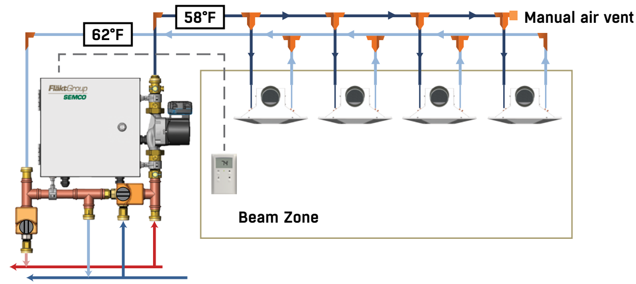
FIGURE 13. Typical zone piping layout as reference for example
