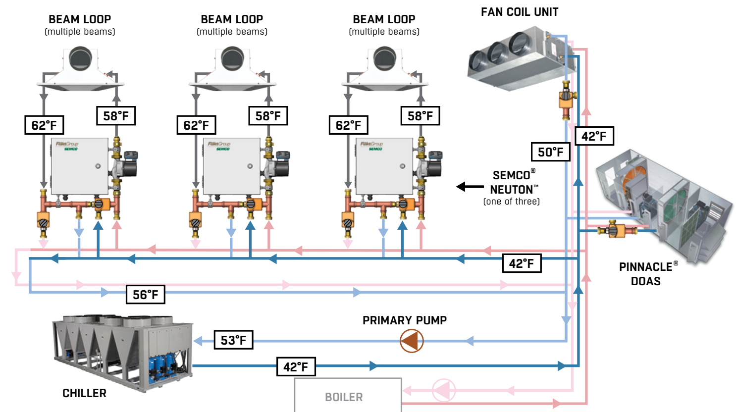
FIGURE 8. Advanced NEUTON® piping scheme (2 pipe approach - cooling primary loop highlighted)
