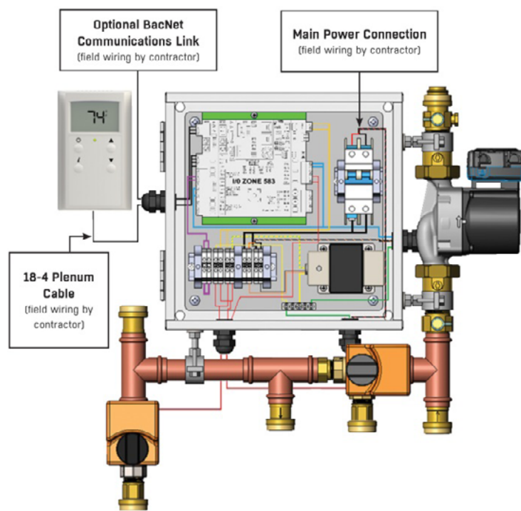
FIGURE 4. Basic control scheme
