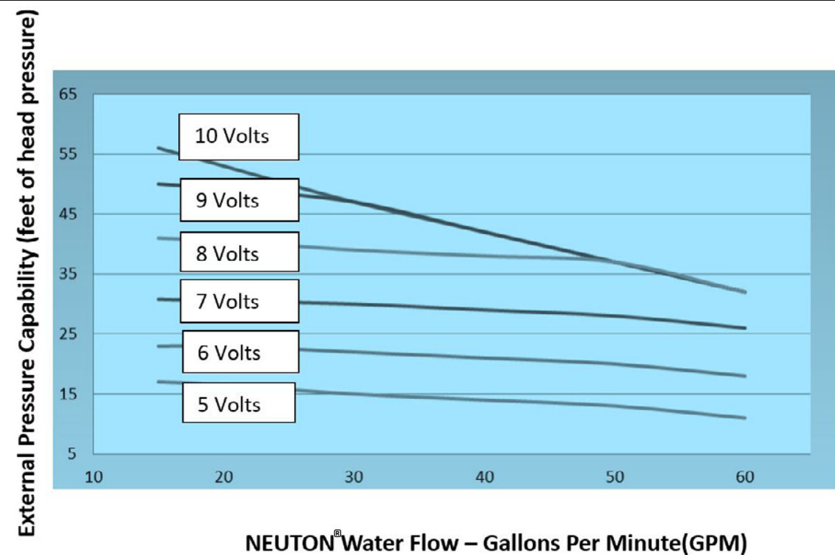
FIGURE 12. Capacity curves for NEUTON® CCBPM-11 and CCBPM-30 at various pump speeds
