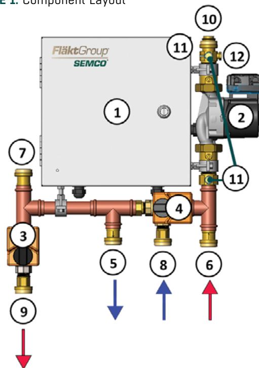
FIGURE 1. Component Layout
