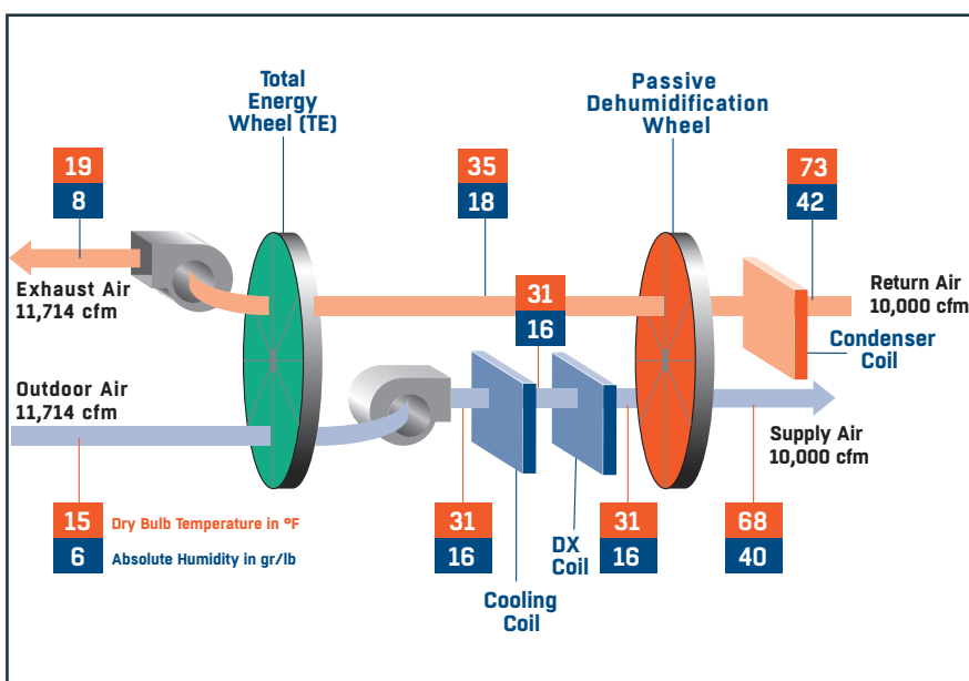
FIGURE 3 Operating in heating mode providing 573 MBtuh of energy and 231,000 MBtuh of free humidification.
