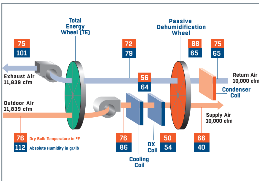
FIGURE 2 Operating at part-cooling load providing 42 tons of total cooling at a SHR of 0.18 using only 30.6 tons of refrigeration input. An equivalent conventional system would require 72.1 tons of cooling and 260 MBtuh of reheat to achieve the same leaving cooling coil temperature, yet without being able to deliver the same dew point of 42.3°F.
