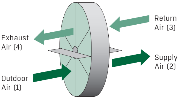
FIGURE 5. Definition of the psychrometric subscripts refer to the following airstreams.
