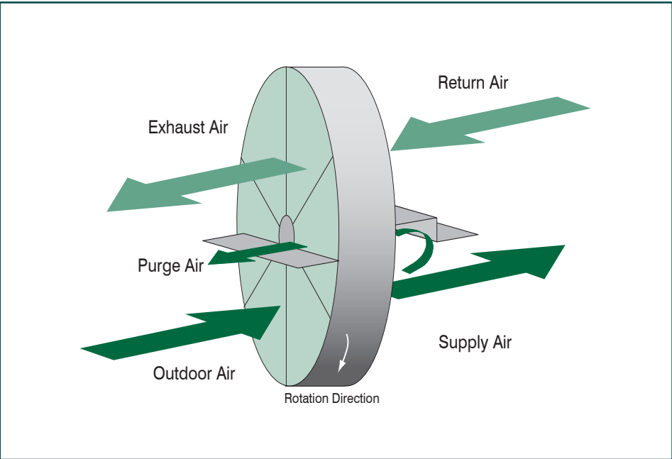
FIGURE 7. Schematic of the purge operation.
