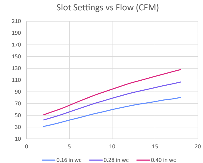
FIGURE 8. 6' Aurora IQSA — Slot Settings vs. Flow (CFM)
