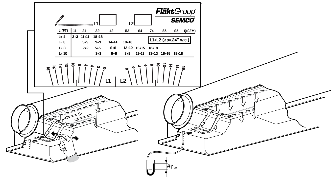
FIGURE 2. Aurora IQSA nozzle adjustment and pressure check
