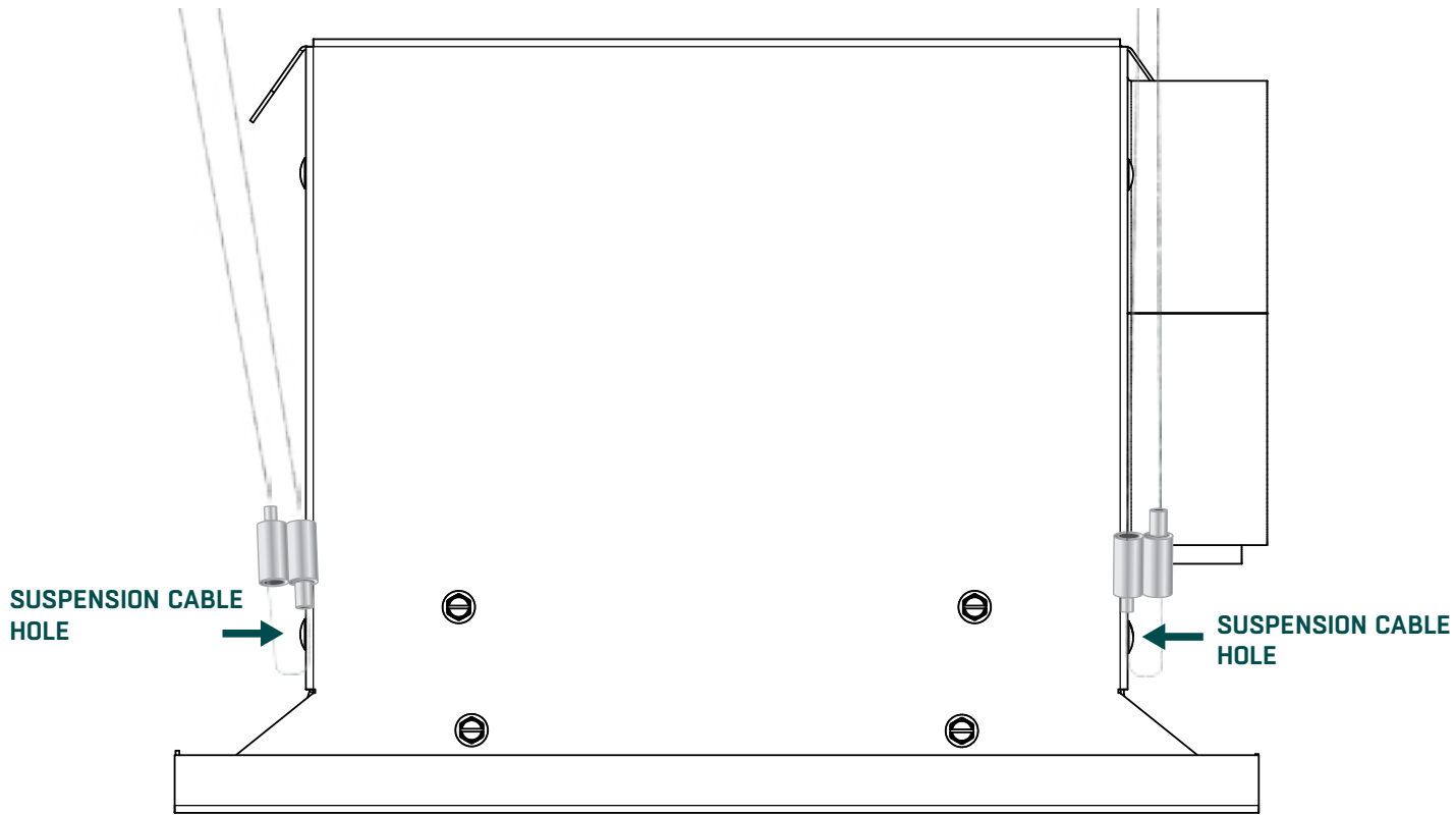
FIGURE 5. Aurora IQSA side view with suspension cables
