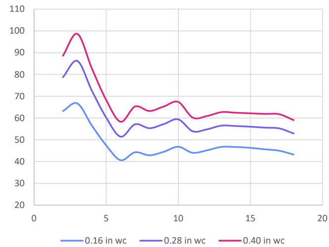
FIGURE 20. 6' Aurora IQSA — Slot Setting vs. Sound (dBA)
