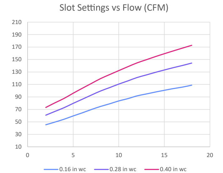
FIGURE 9. 8' Aurora IQSA — Slot Settings vs. Flow (CFM)
