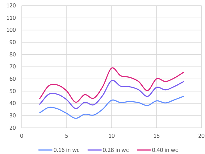
FIGURE 19. 4' Aurora IQSA — Slot Setting vs. Sound (dBA)
