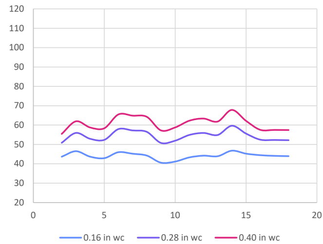
FIGURE 21. 8' Aurora IQSA — Slot Setting vs. Sound (dBA)
