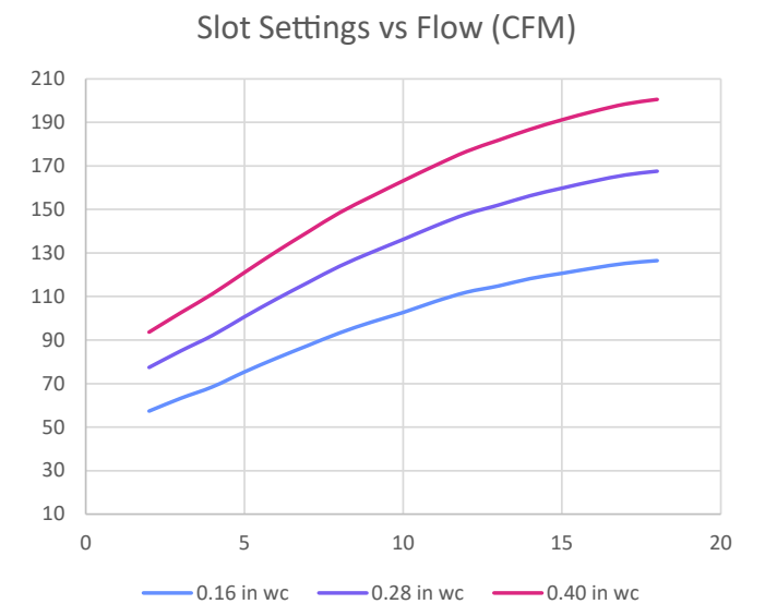
FIGURE 10. 10' Aurora IQSA — Slot Settings vs. Flow (CFM)
