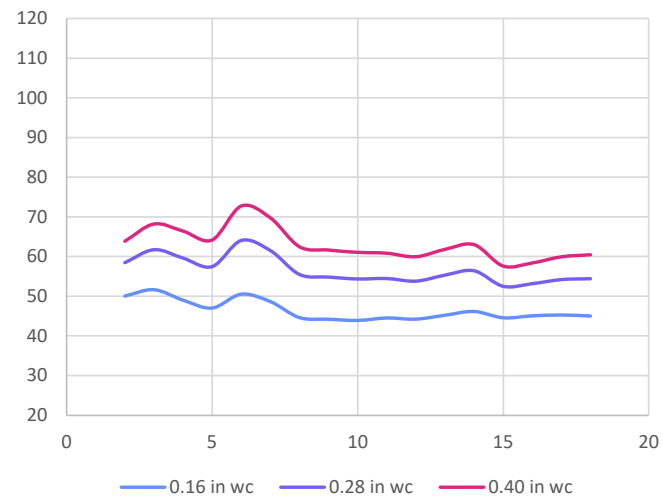
FIGURE 22. 10' Aurora IQSA — Slot Setting vs. Sound (dBA)
