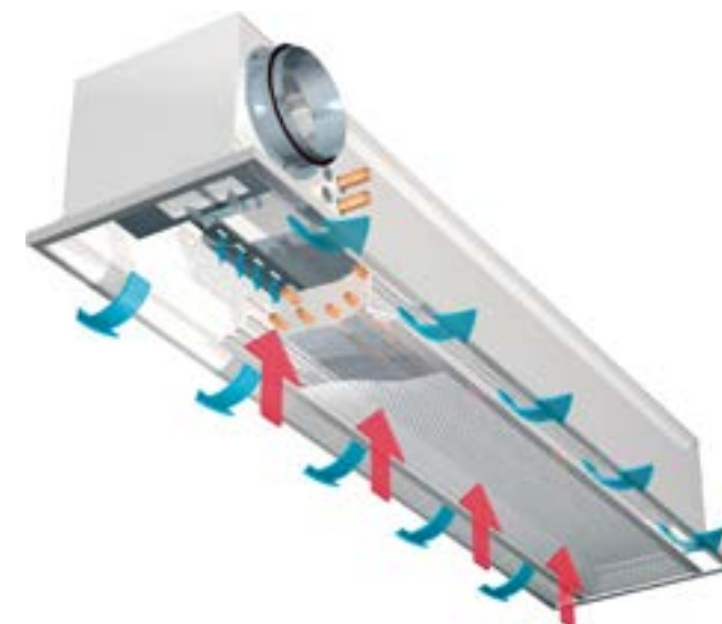
FIGURE 3. The Aurora IQSA air flow distribution
