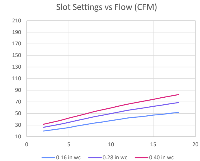
FIGURE 7. 4' Aurora IQSA — Slot Settings vs. Flow (CFM)
