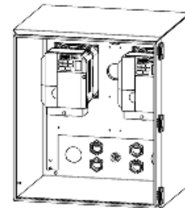
FIGURE 4. VFD Enclosure
